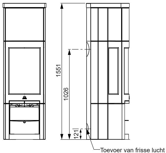
Jøtul F 377 Advance met High Top
